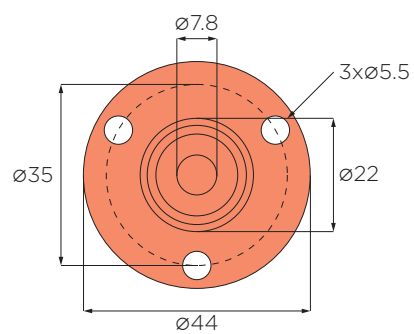
A FLANGE (STANDARD)
