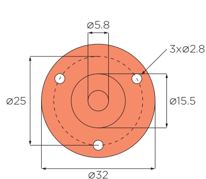
A FLANGE (STANDARD)
