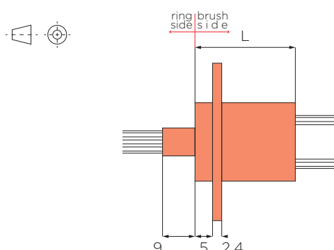
SVTS A 03 | SVTS A 06
