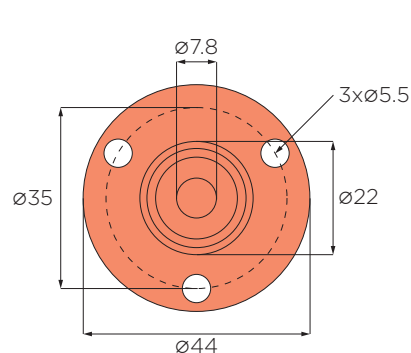
A FLANGE (STANDARD)
